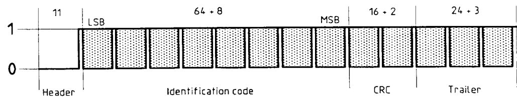
Figure 2 — Structure of the FDX identification telegram
