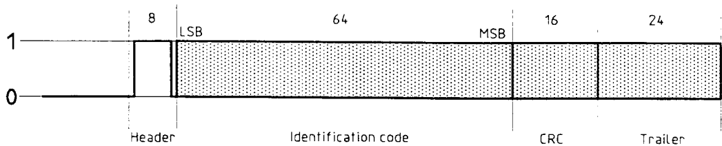
Figure 5 — Structure of the HDX identification telegram
