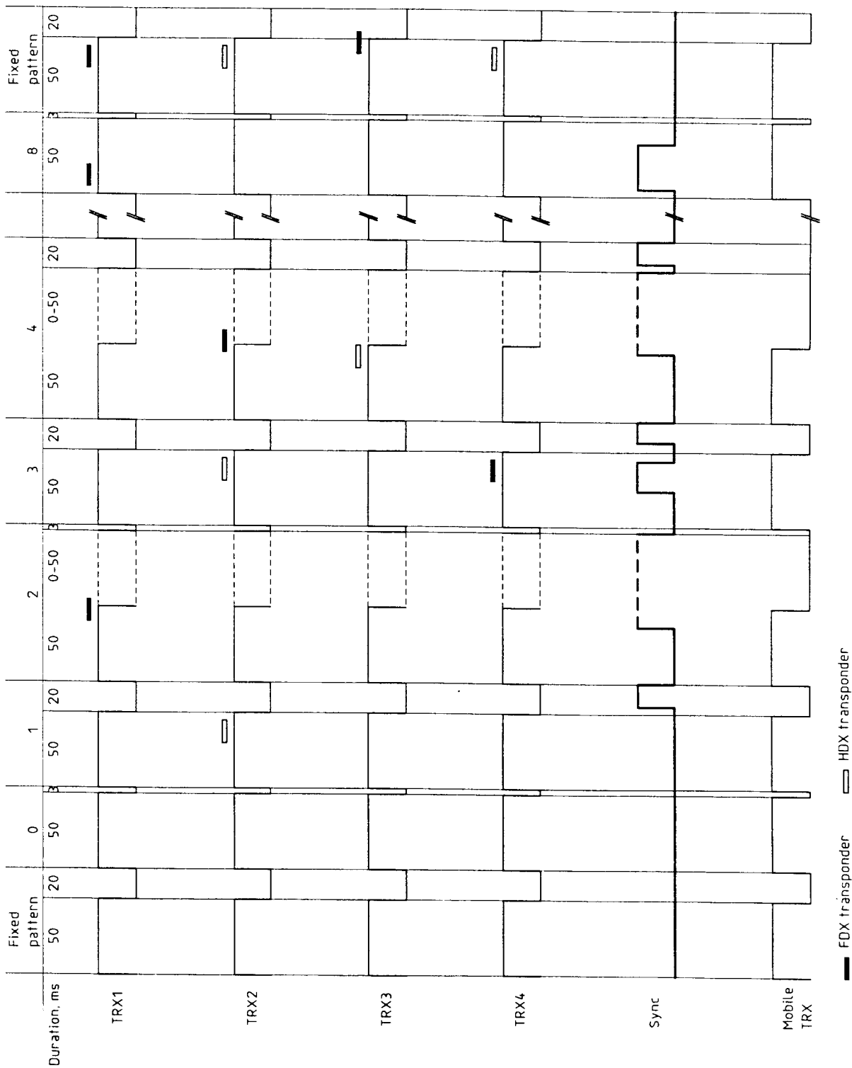
Figure C.1 — Interrogation protocol patterns
